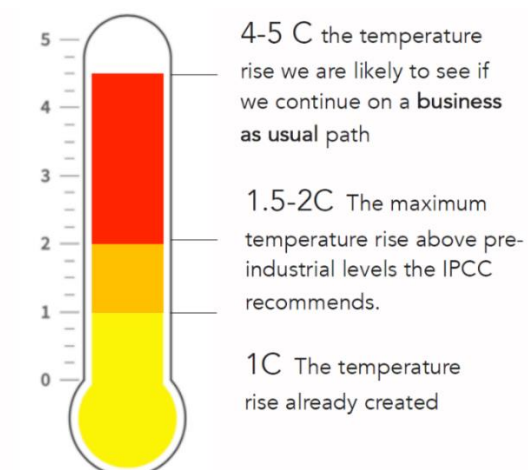
Figure 6: Special Report on 1.5C by IPCC, and diagram of the potential range of climate change to 2100 (Diagram credit: Etude, 2021).
