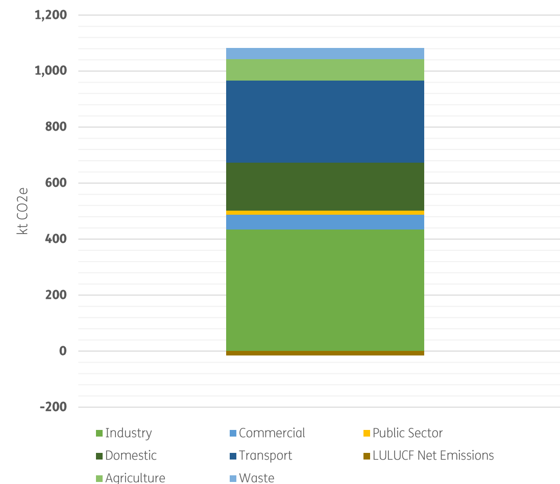
Figure 10: Sectoral emissions trajectories in Swale for 2022 – BEIS/DESNZ UK local authority greenhouse gas emissions (2024).
