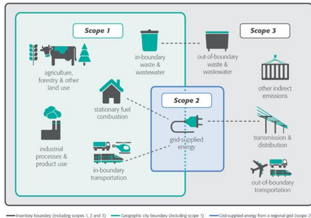
Figure 1: Various Sources of emissions according to Scope 1, 2 and 3.
