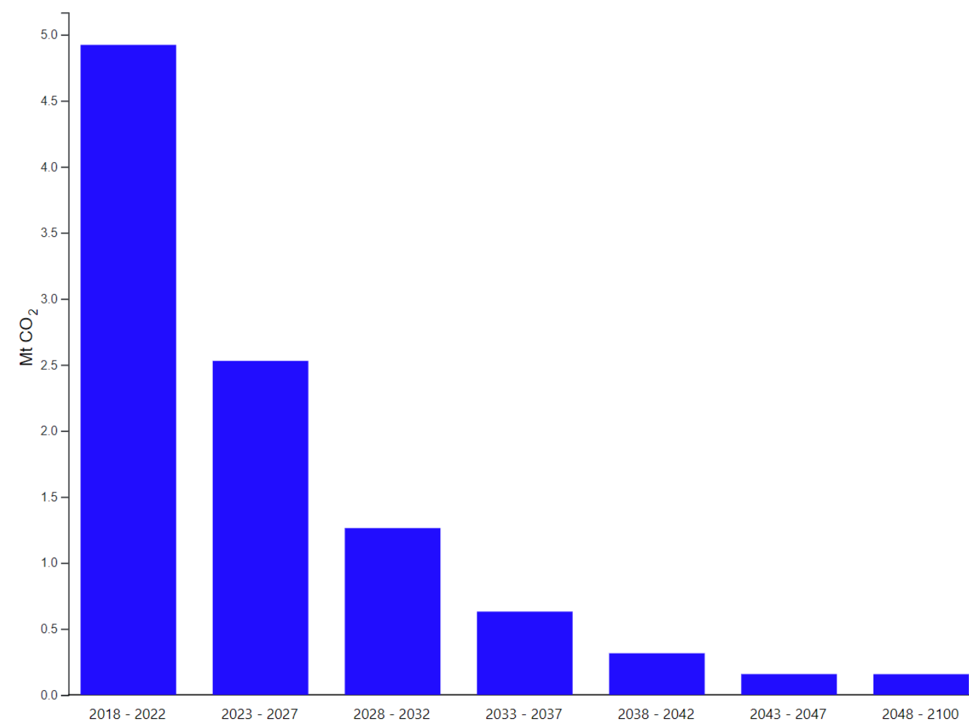
Figure 2: Swale carbon budgets to 2100 (energy-only, CO 2 only) compliant with the UK's commitment to the Paris Agreement. Calculated by the Tyndall Centre. [viii]
