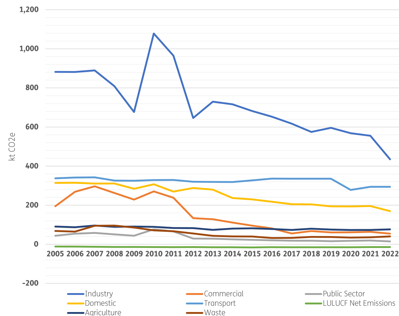
Figure 9: Sectoral emissions trajectories in Swale from 2005-2022 – BEIS/DESNZ UK local authority greenhouse gas emissions (2024).
