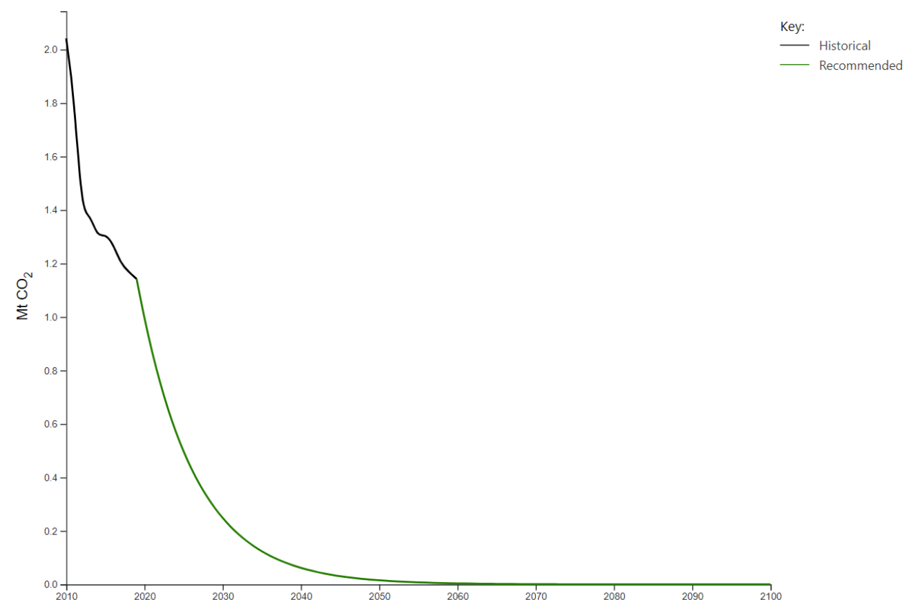
Figure 11: Emissions reduction pathway for energy-only CO 2 emissions to fulfil carbon budgets for Swale from 2018 to 2100 compatible with the Paris Agreement. Tyndall Centre (2024).
